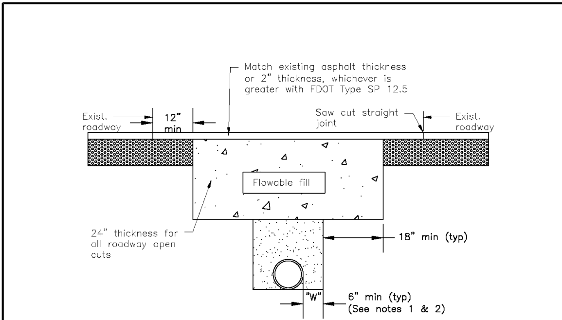
Figure 50 - Roadway Open Cut Detail (US-63)
