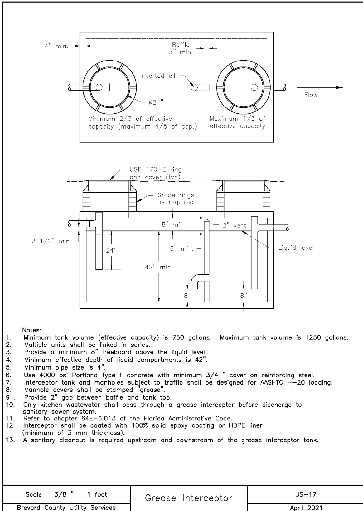
Image Description US-17 Grease Interceptor
