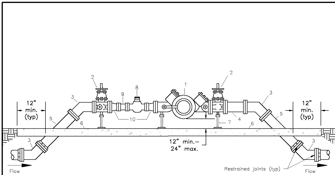
Figure 41 - Backflow Preventer with Meter for Fire Services 3" to 8" Detail (US-47)
