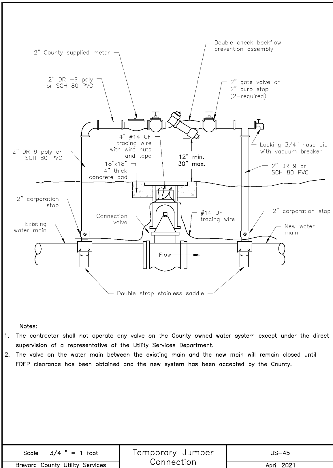
Image Description US-45 Temporary Jumper Connection
