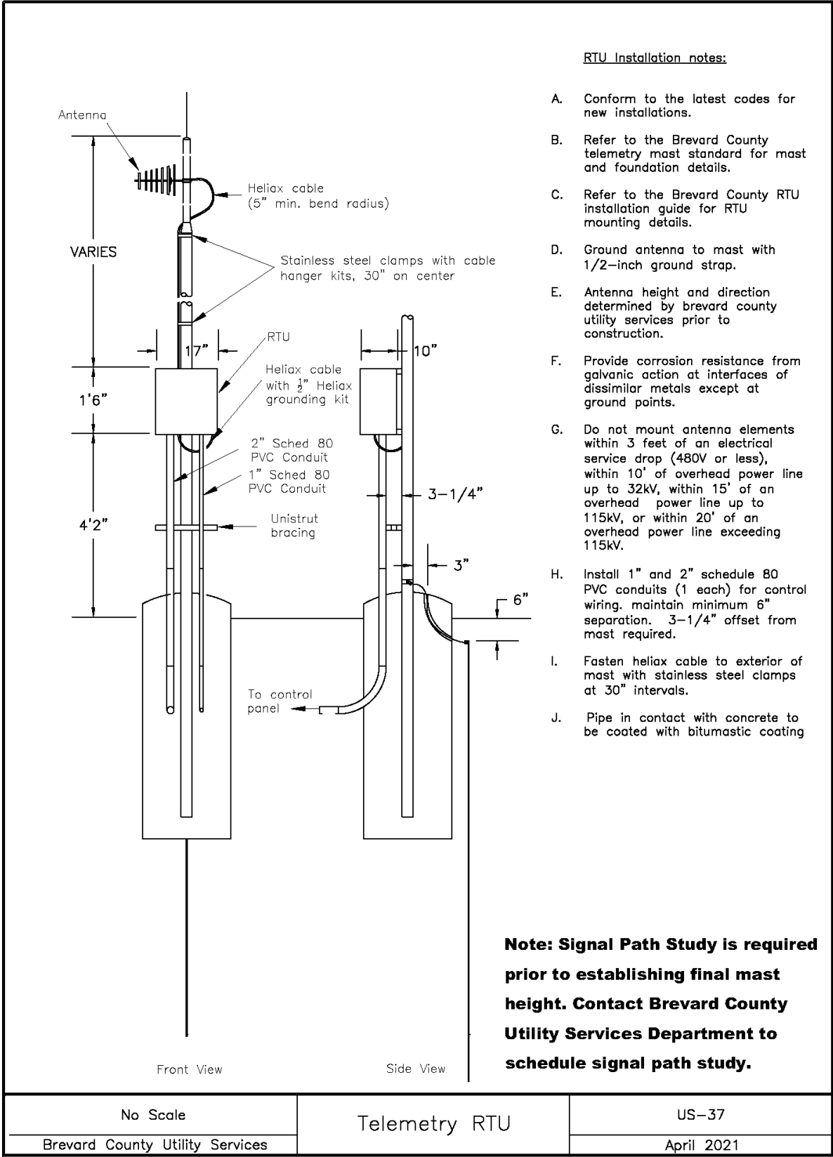
Image Description US-37 Telemetry RTU
