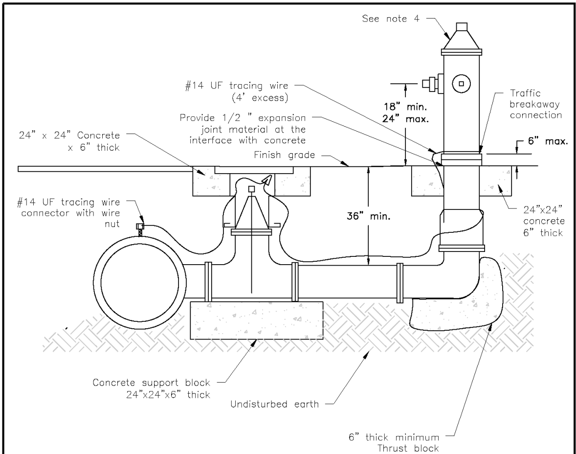
Figure 37 - Fire Hydrant Assembly Detail (US-43)
