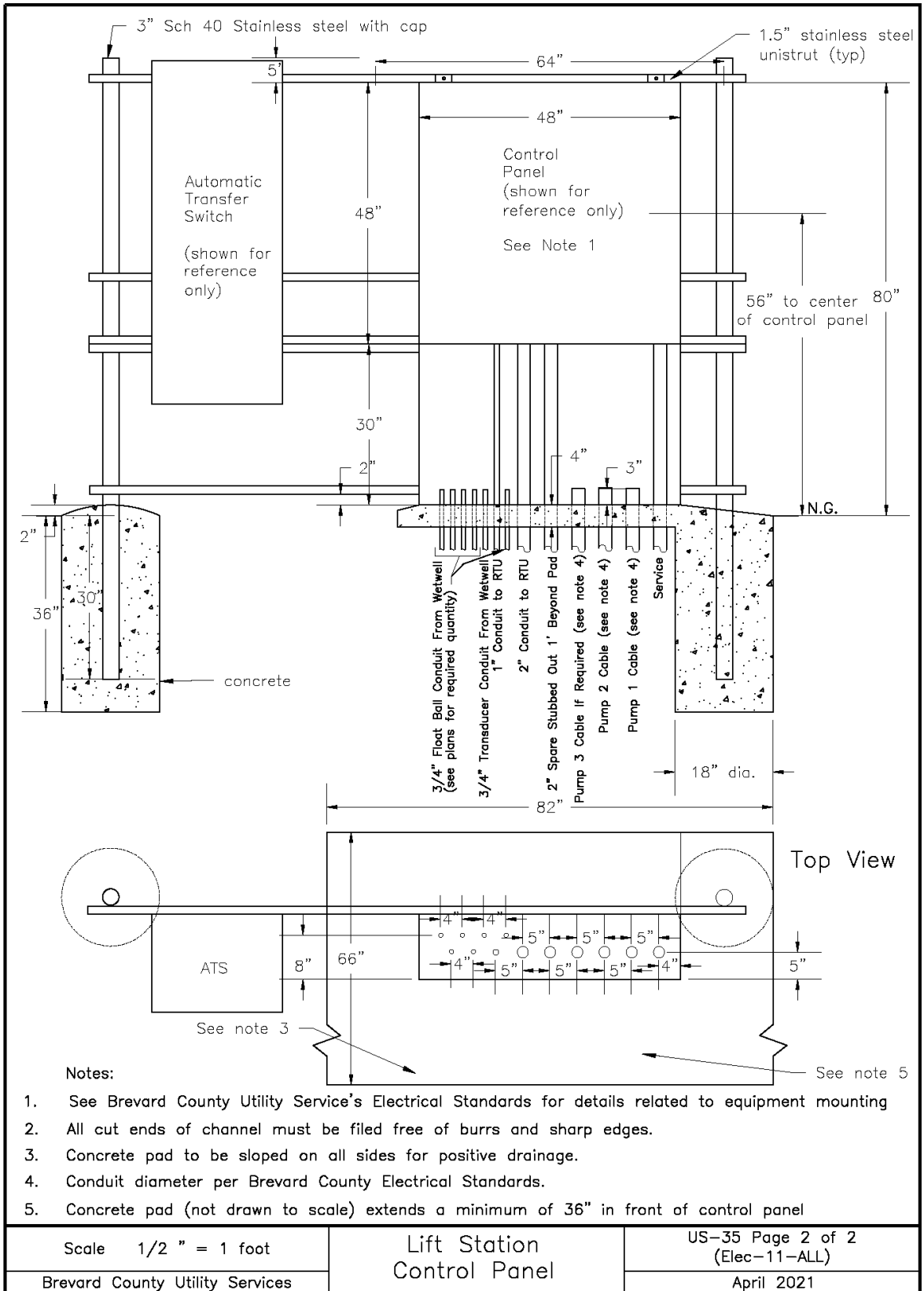
Image Description US-35 Page 2 of 2 (Elec-11-ALL) Lift Station Control Panel
