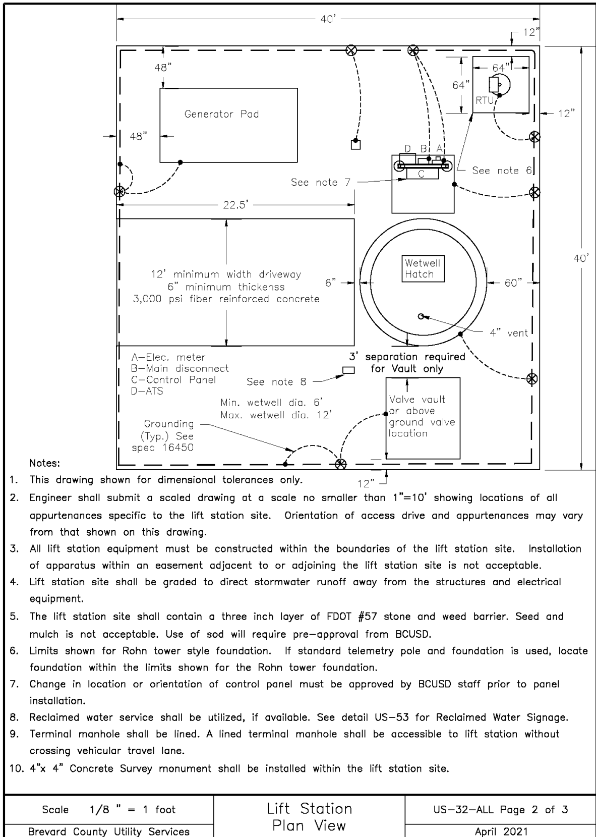
Figure 24 - Lift Station Plan View Detail (US-32-ALL Page 2 of 3)
