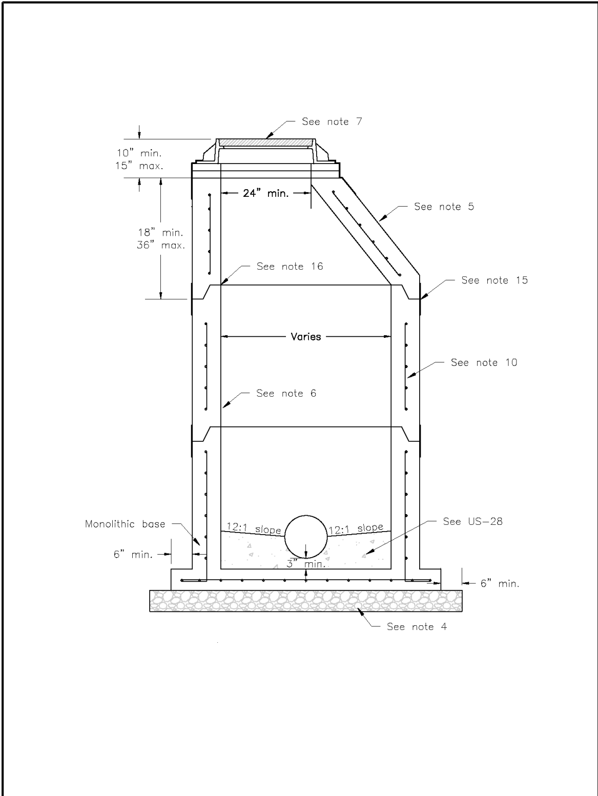
Figure 12 - Eccentric Manhole Detail (US-22)
