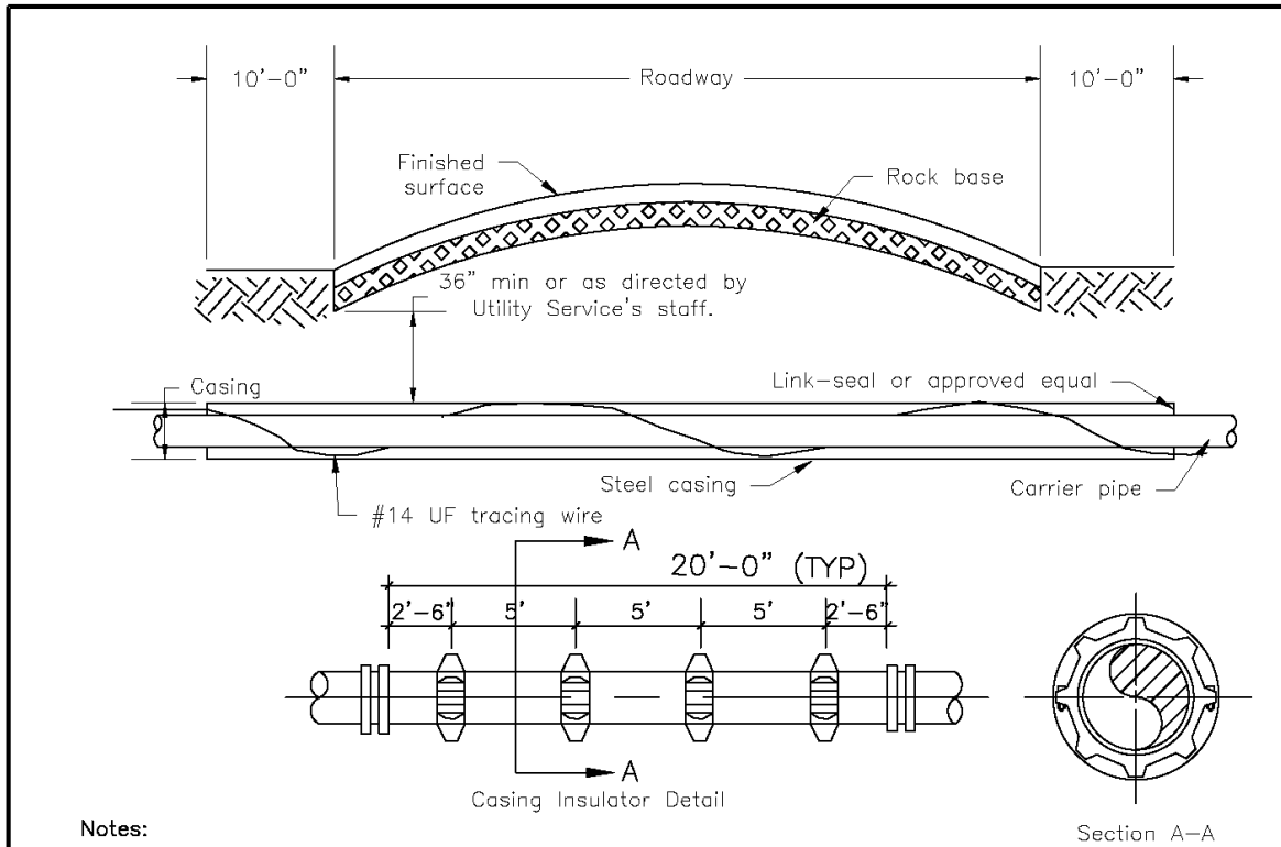
Figure 57 - Casing Installation Detail (US-70)
