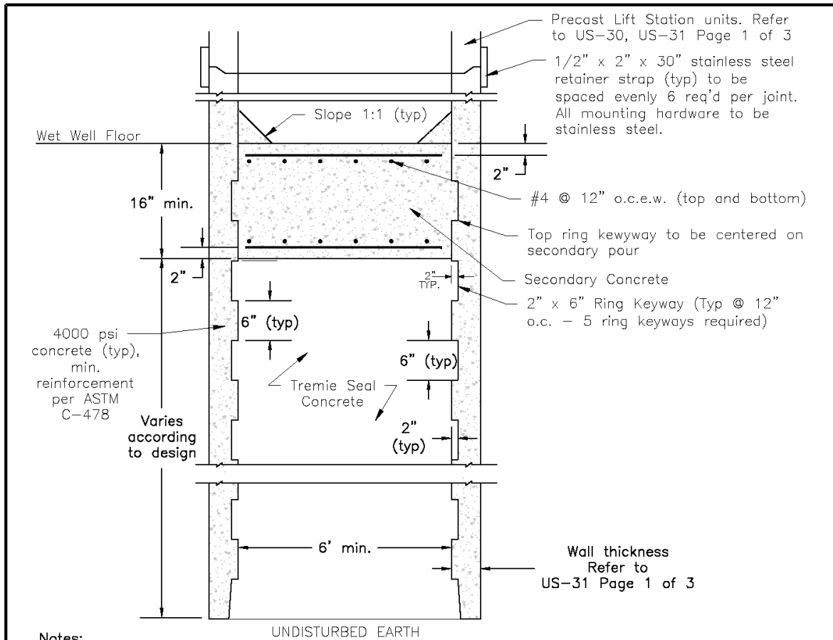
Figure 21 - Tremie Wet Well Installation Detail (US-31 Page 2 of 3)
