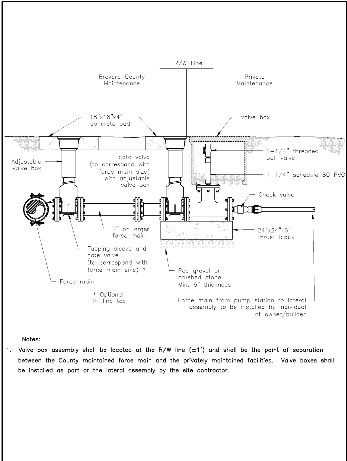
Figure 5 -Private/Public Force main Transition (US-14)
