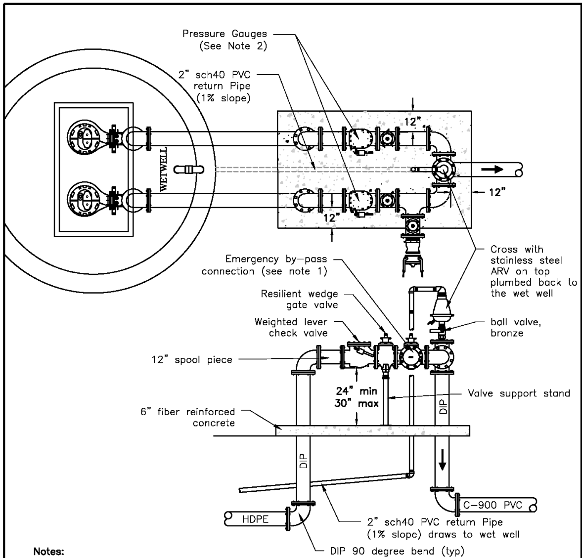
Figure 26 - Lift Station Above Ground Valving Detail (US-33)
