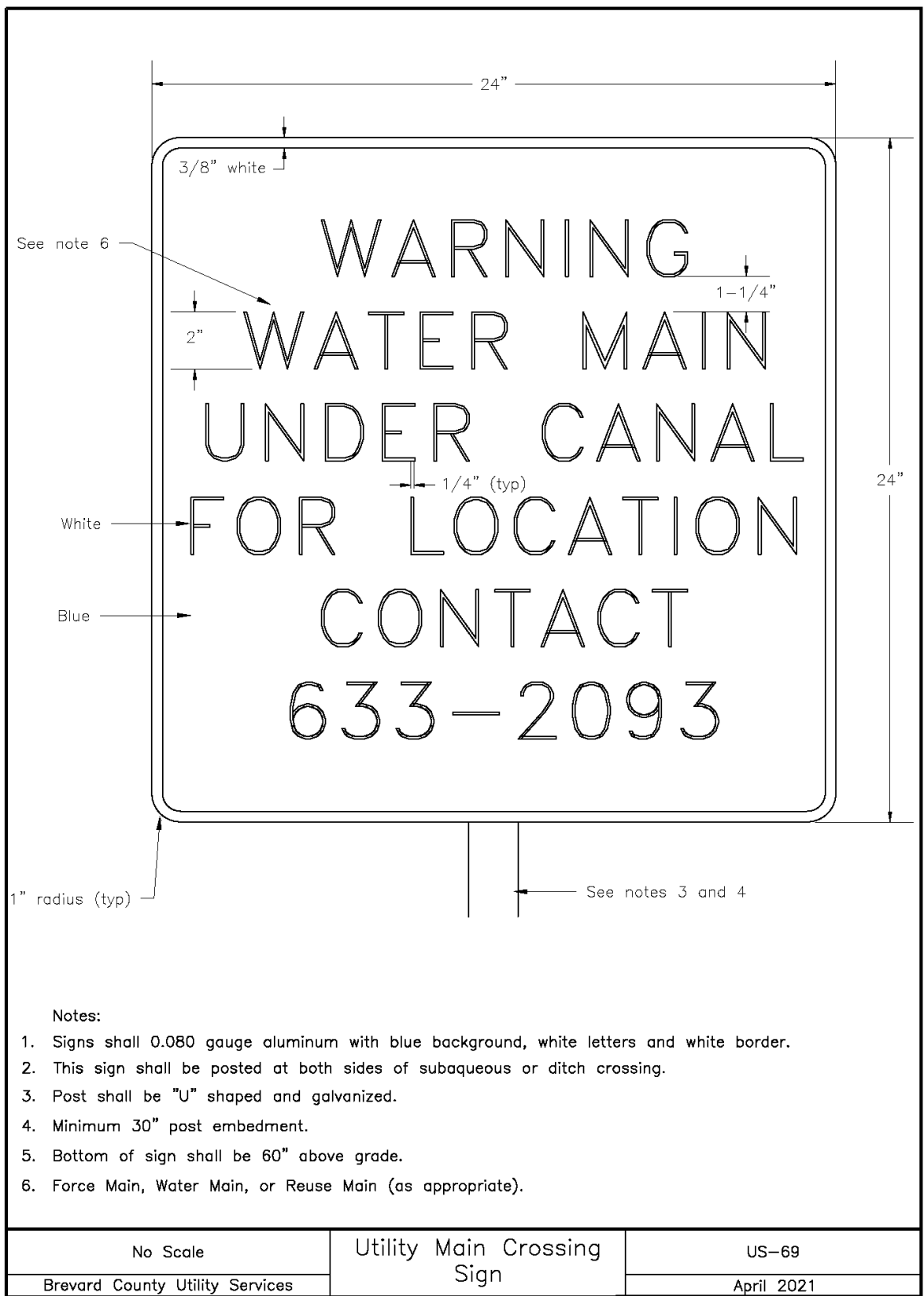
Image Description US-69 Utility Main Crossing Sign
