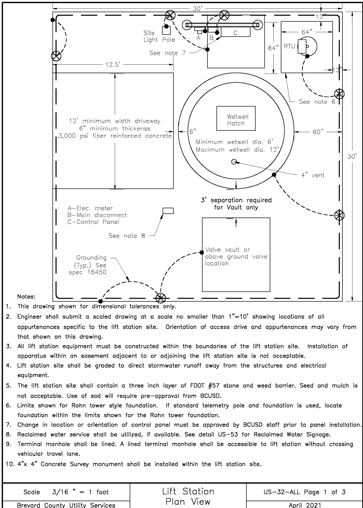
Figure 23 - Lift Station Plan View Detail (US-32-ALL Page 1 of 3)
