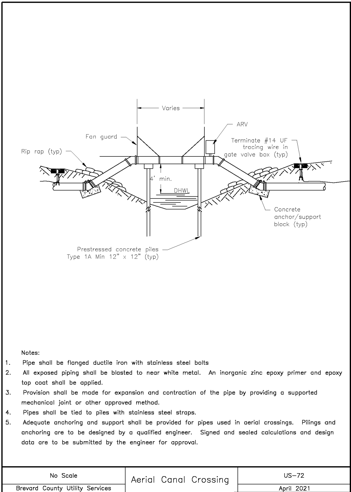
Figure 59 - Aerial Canal Crossing Detail (US-72)
