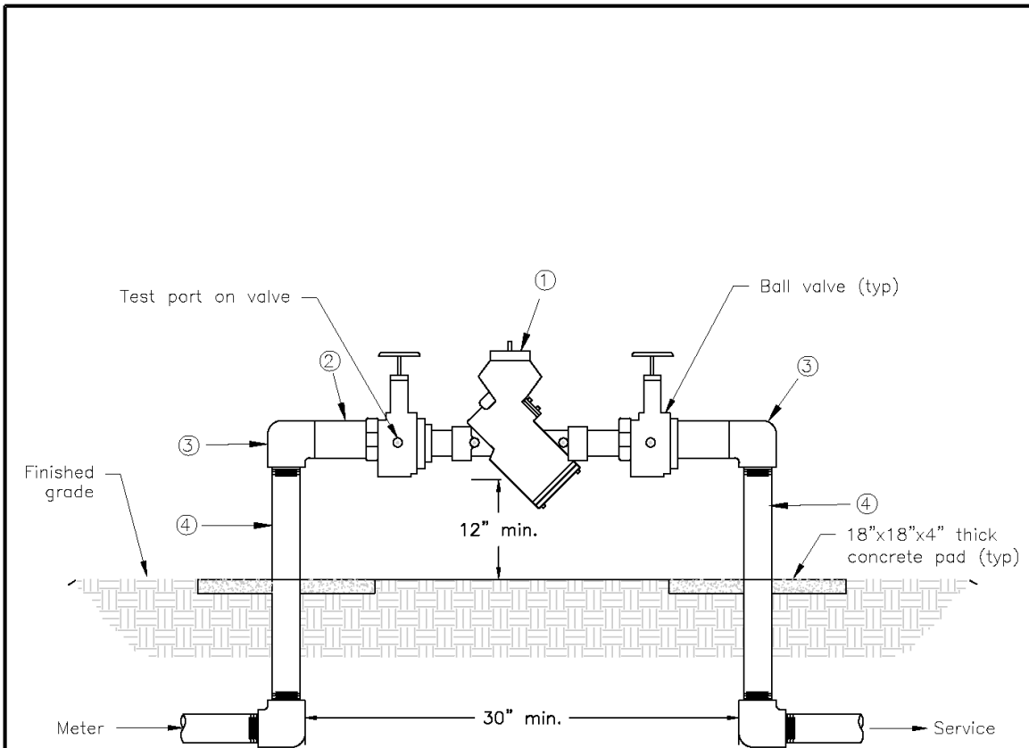
Figure 40 - 3/4" to 2" Backflow Preventer Detail (US-46)
