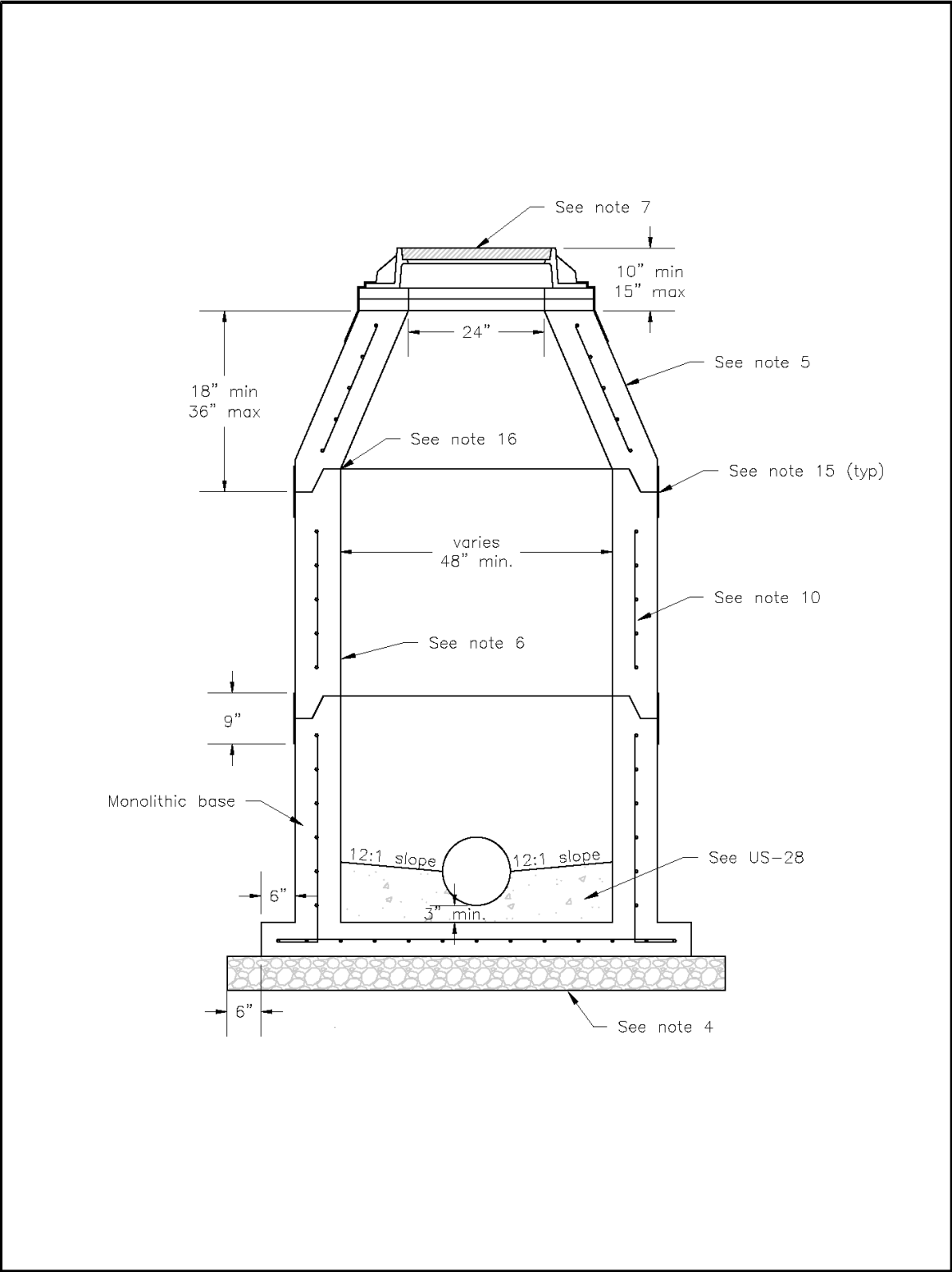
Figure 11 - Concentric Manhole Detail (US-21)
